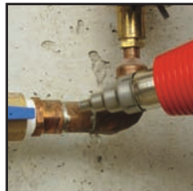
Solder Copper Pipe
