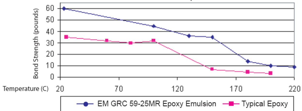
Helical Coil Bond vs. Temperature
